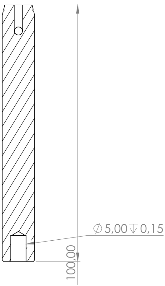
SECTION B-B
