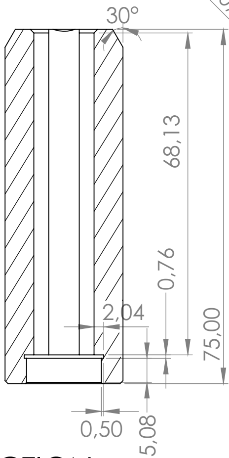
SECTION B-B
